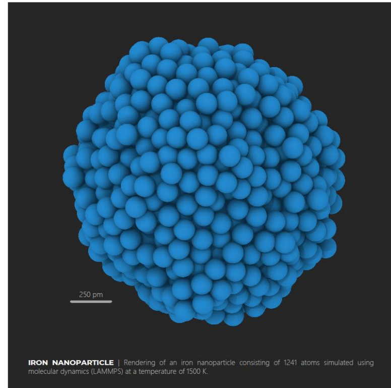
3 rd Place: Rendering of an Iron Nanoparticle Consisting of 1241 Atoms Simulated Using Molecular Dynamics, Timothy Sipkens University of British Columbia
